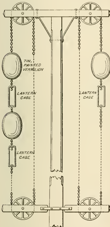
OLD BALL AND LAMP SIGNAL AT TERMINALS.
